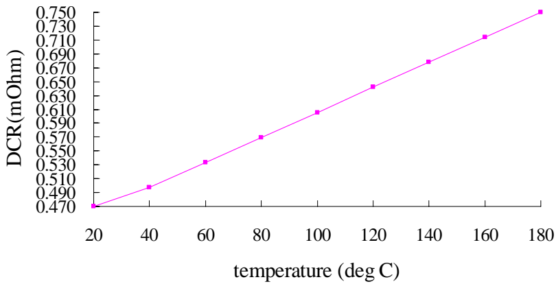
DCR VS temperature
