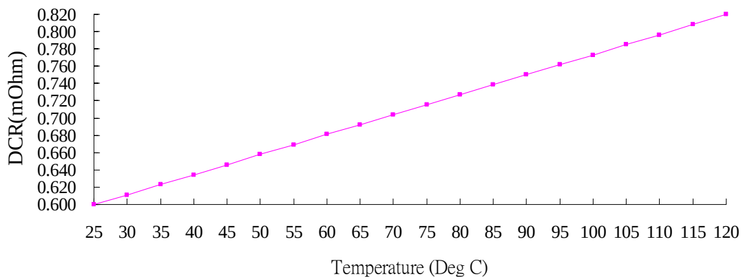
Temperature VS DCR
